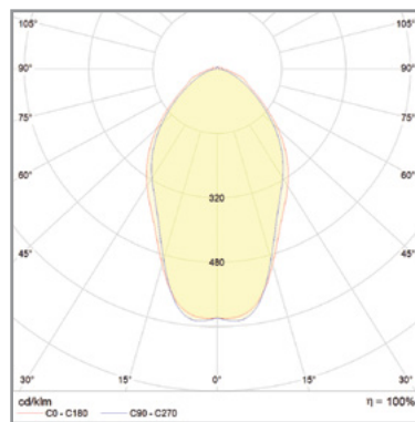
Medium beam 60°
