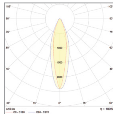
Narrow beam 30°
