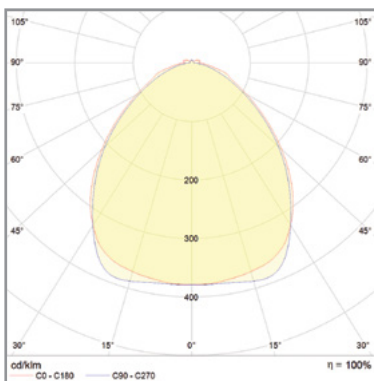
Wide beam 90°
